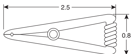
Clip-On Heat Sink
