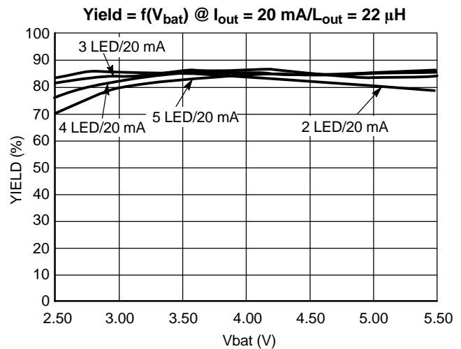
Figure 13. Overall Efficiency vs. Power Supply @ I_{out} = 20\text{ mA} , L = 22\text{ }\mu\text{H}
