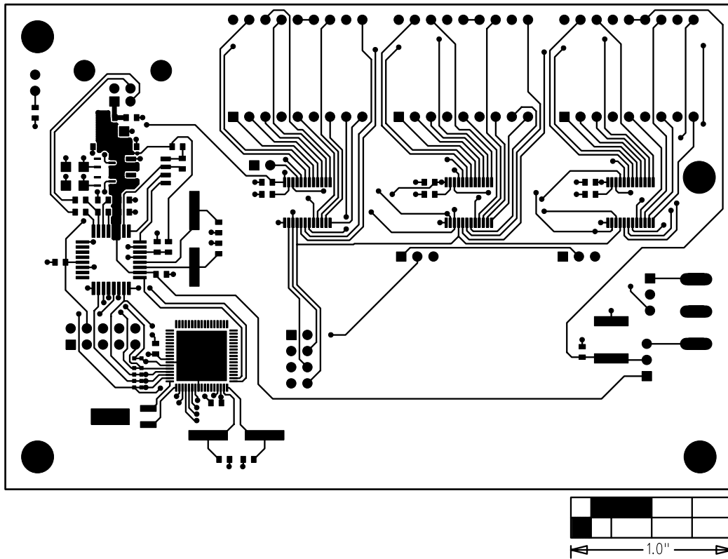
Figure 5. MAX6969 EV Kit PCB Layout—Component Side
