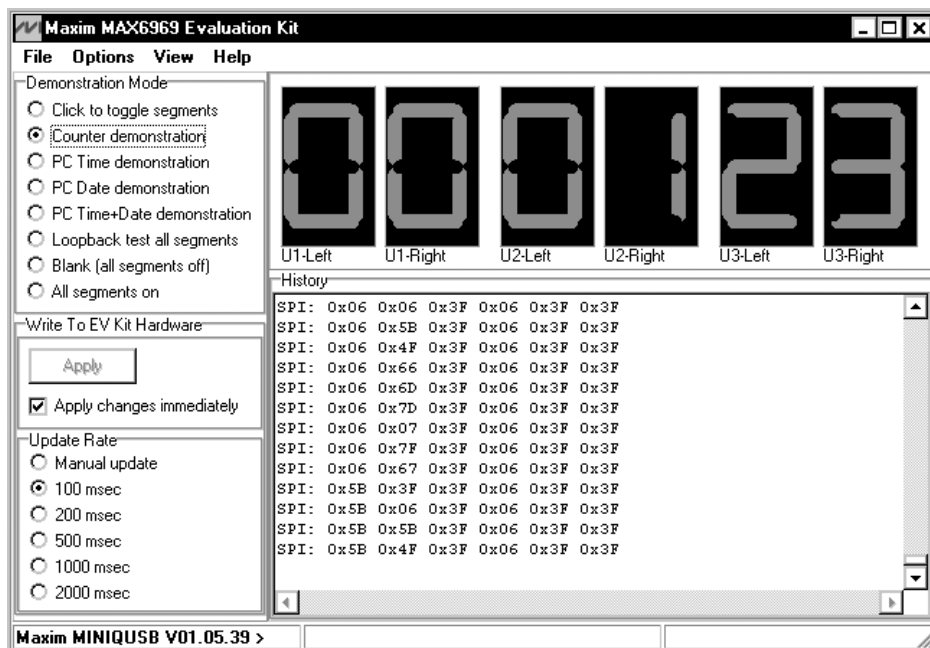
Figure 1. The MAX6969 EV Kit Software's Counter Demonstration (shows the 7-segment display counting up in decimal)
