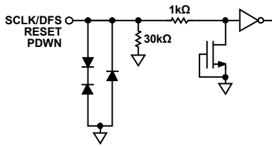
Figure 8. Equivalent SCLK/DFS, RESET, PDWN Input Circuit
