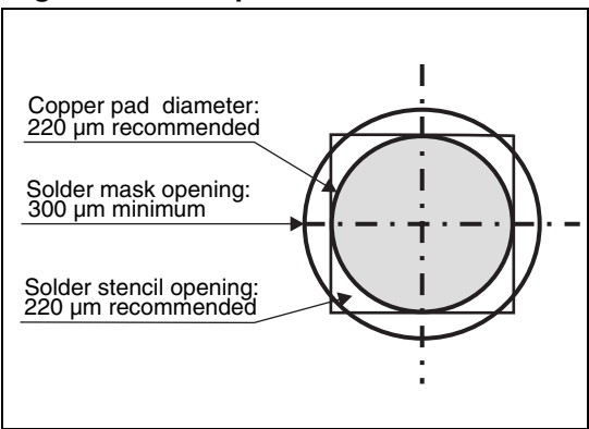
Figure 12. Footprint
