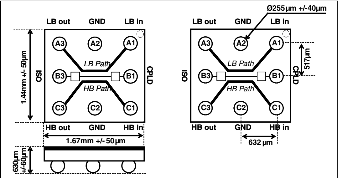
Figure 11. Package dimensions
