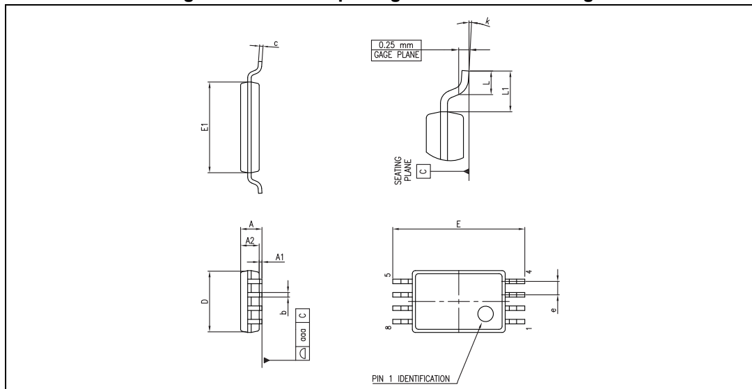
Figure 16. TSSOP8 package mechanical drawing
