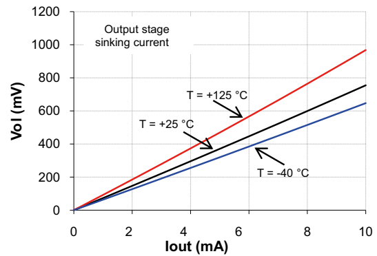
Figure 10. Output stage high-state saturation voltage vs. output current (Vsense = +1 V)
