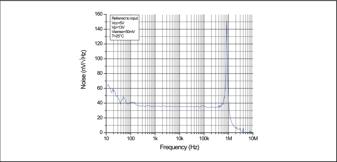
Figure 15. Noise level
