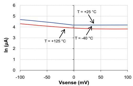
Figure 8. Vn pin input current vs. Vsense
