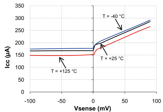
Figure 6. Supply current vs. V_{sense}
