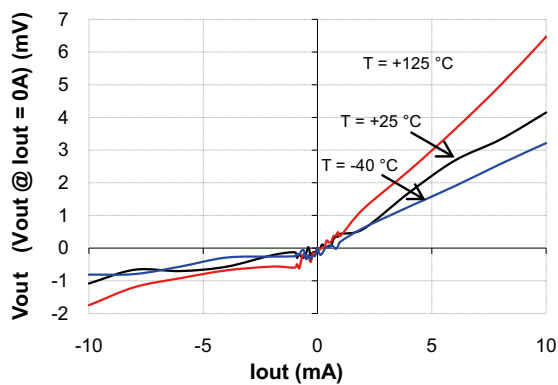
Figure 11. Output stage load regulation
