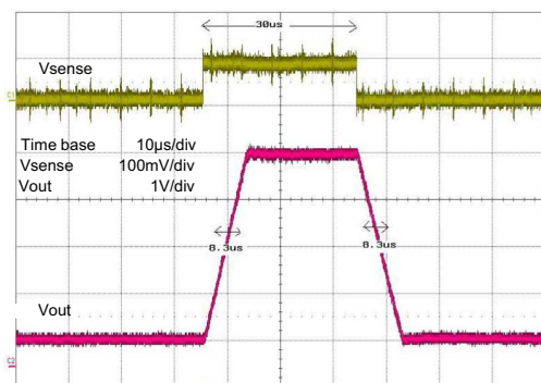
Figure 12. Step response
