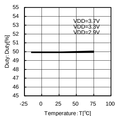
Fig.77 18.4MHz Temperature - Duty
