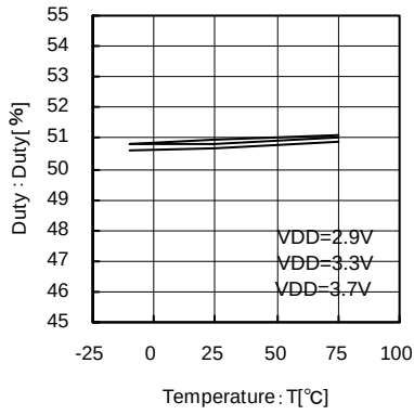
Fig.34 16.9MHz Temperature—Duty
