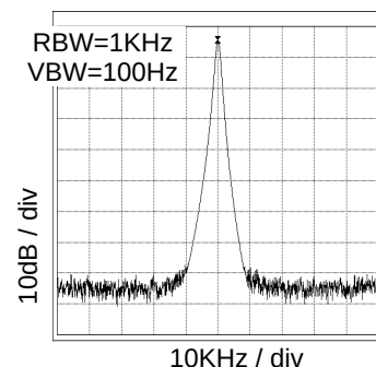
Fig.49 27MHz Spectrum VDD=3.3V, at CL=15pF
