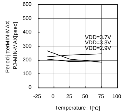
Fig.30 13.5MHz Temperature - Period-Jitter MIN-MAX
