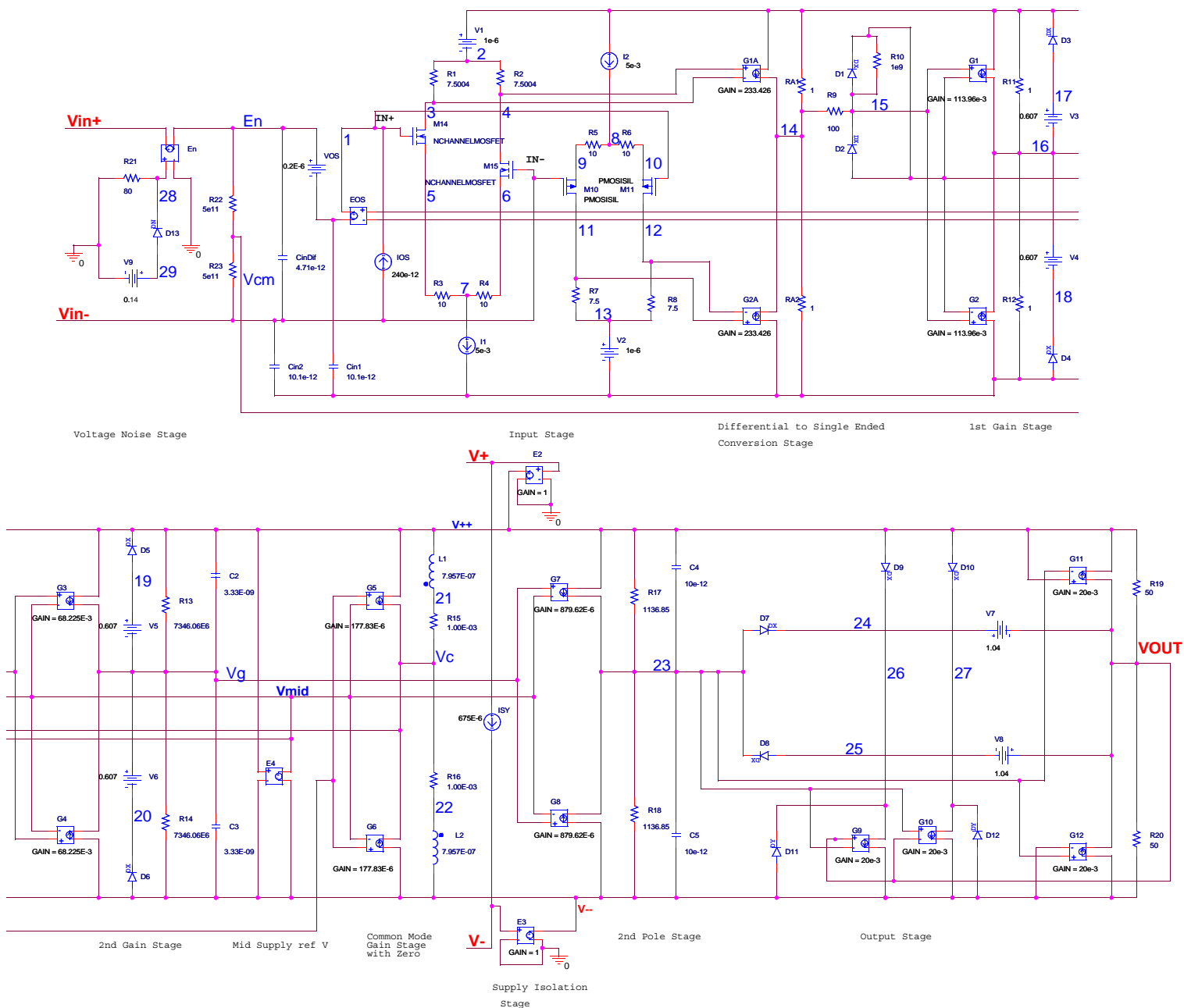
FIGURE 48. SPICE SCHEMATIC
