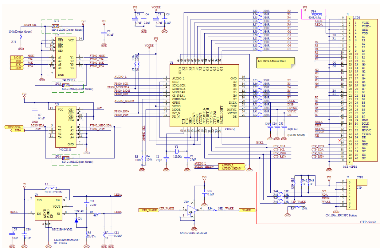
Figure 3-1 - VM801B43A/VM801B50A (4.3"/5.0" Version)
