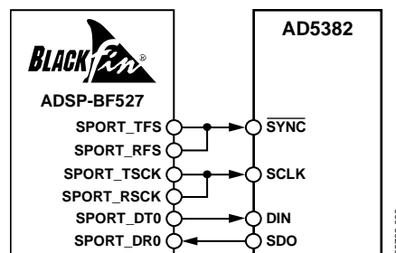
Figure 37. AD5382-to-ADSP-BF527 Interface
