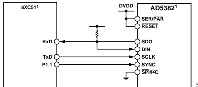
Figure 36. AD5382-to-8051 Interface
