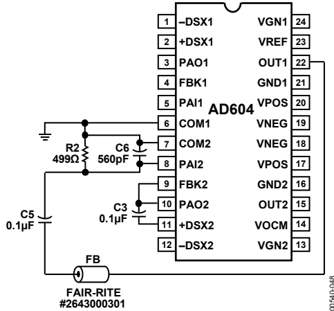
Figure 48. Modifications of the AGC Amplifier to Create 96 dB of Gain Range
