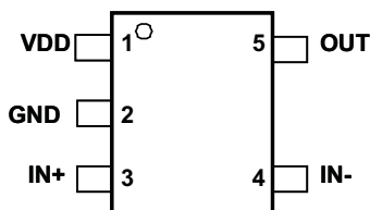
UCC27517A-Q1 DBV (Top View)
