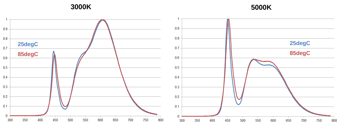
Fig 1. Relative Spectrum of Emission at typical current.
