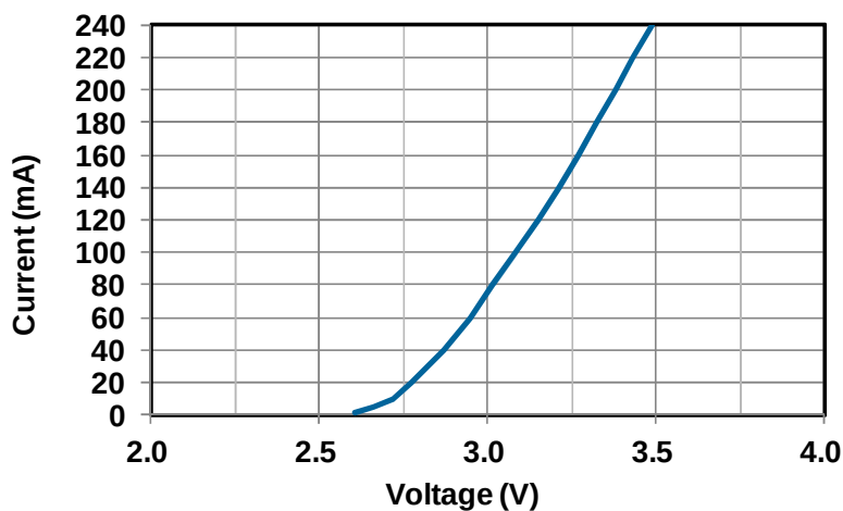
Fig 3. Forward Current vs. Forward Voltage-Curve
