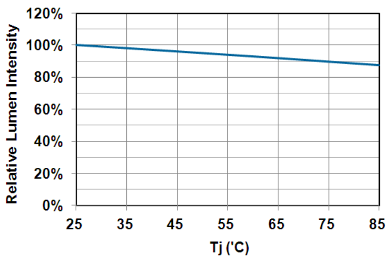
Fig 4. Relative Luminous vs Junction Temperature
