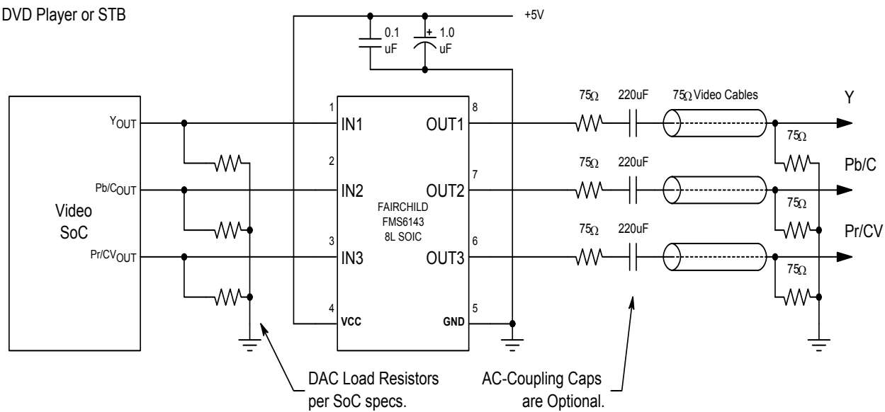
Figure 10. Typical Application
