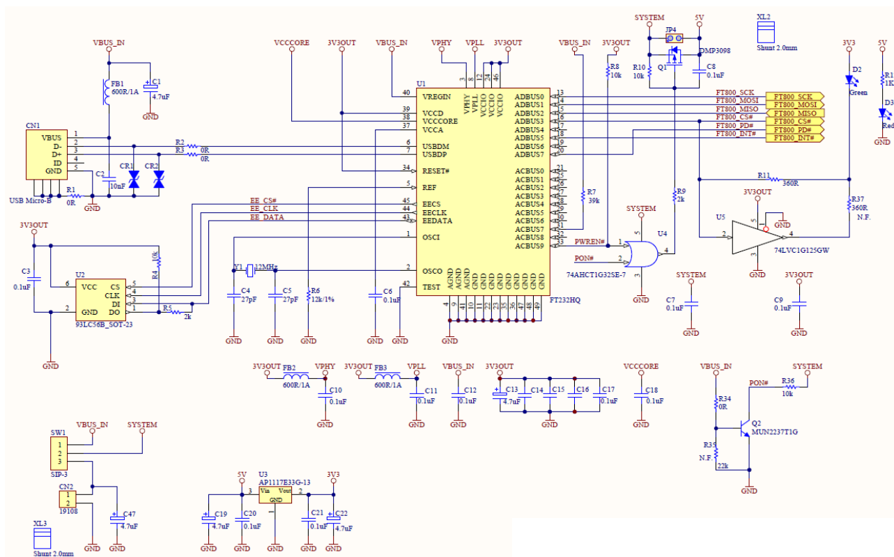
Figure 4-3 – VM800BU SPI Interface and Power Input
