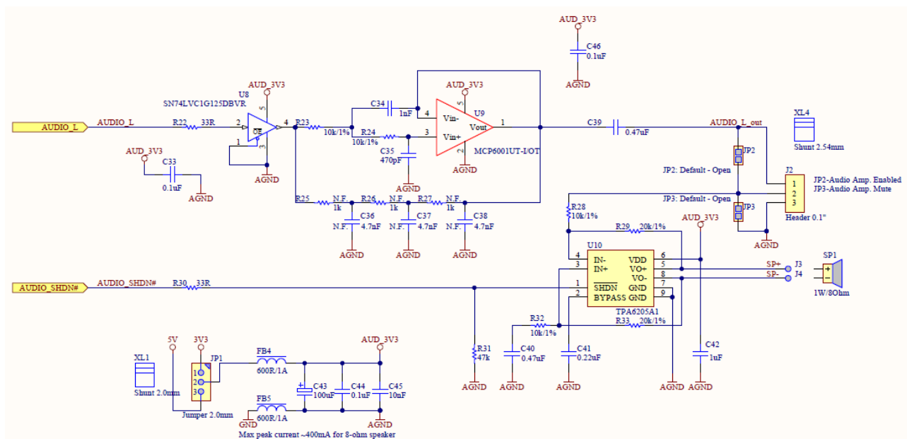
Figure 4-4 – VM800BU Audio Circuits
