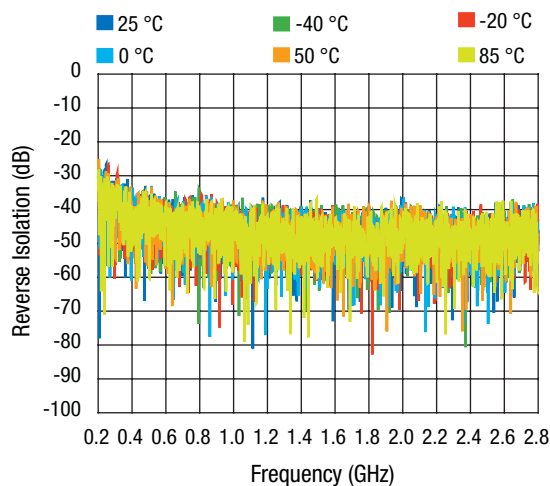
Reverse Isolation vs. Frequency, V_{CC} = 3.5 V P_{IN} = -30 dBm, V_{APC1,2} = 2.7 V
