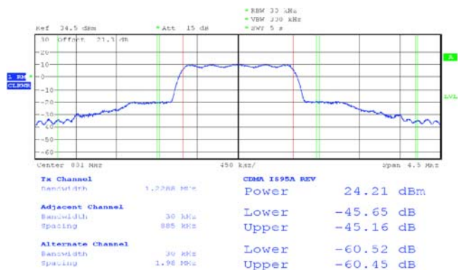
ACPR, IS-95 REV, V_{CC} 3.5 V, V_{APC1, 2} = 2.7 V 881 MHz @ 25 °C
