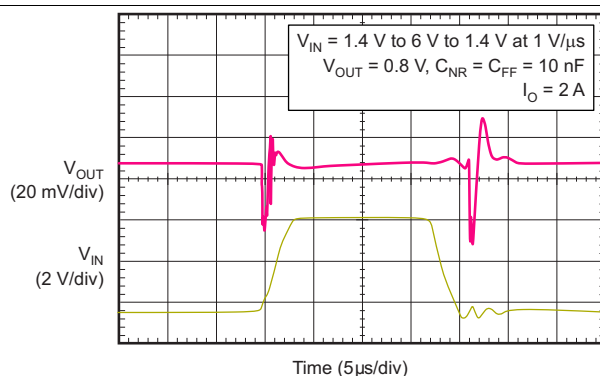
Figure 49. Line Transient
