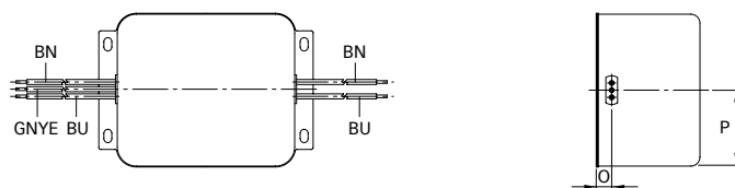
Connection style -08, 25 and 36A types
