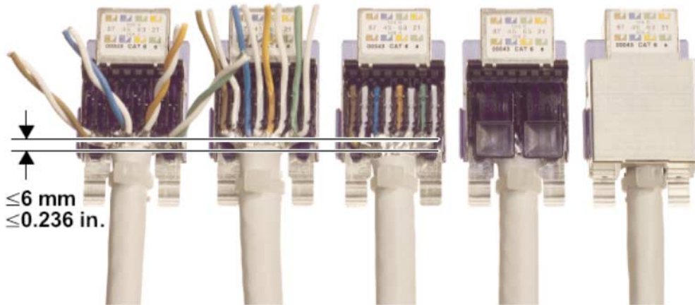
Figure 3 Connecting the conductors to the IDC terminal blocks
