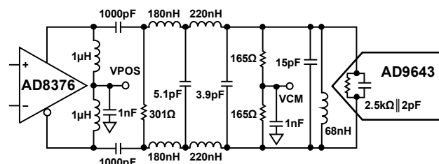
Figure 49. Differential Input Configuration Using the AD8376
