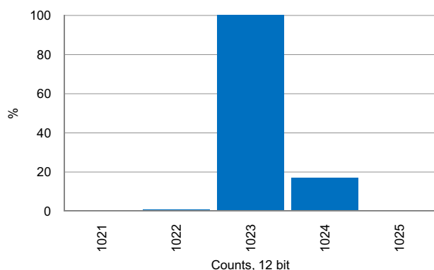
Figure 11-39. SAR ADC Noise Histogram, 100 kps, Internal Reference No Bypass
