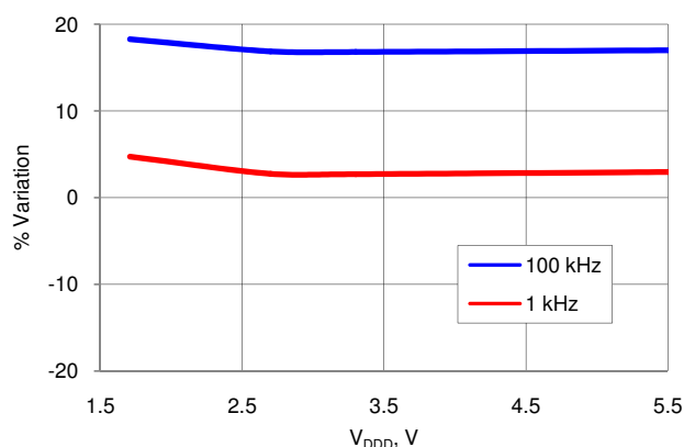
Figure 11-80. ILO Frequency Variation vs. V_{DD}
