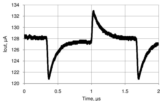
Figure 11-53. IDAC Glitch Response, Codes 0x7F - 0x80, 255 \mu A Mode, Source Mode, Fast Mode, V_{DDA} = 5 V
