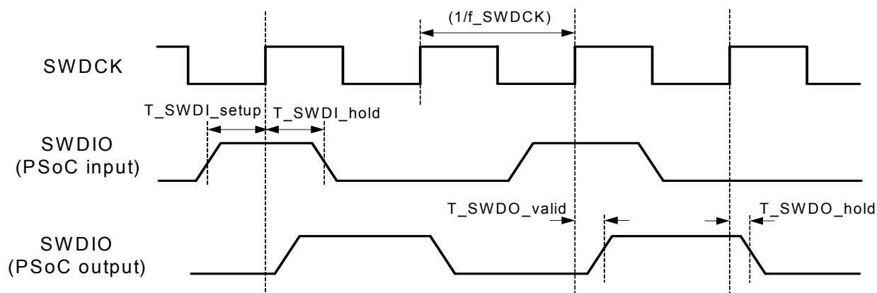
Figure 11-75. SWD Interface Timing
