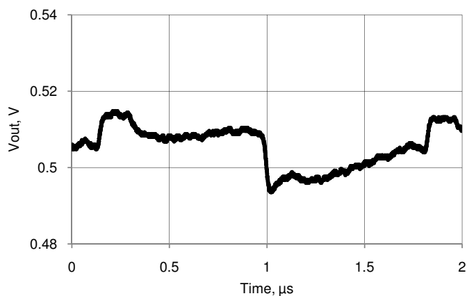
Figure 11-65. VDAC Glitch Response, Codes 0x7F - 0x80, 1 V Mode, Fast Mode, Vdda = 5 V
