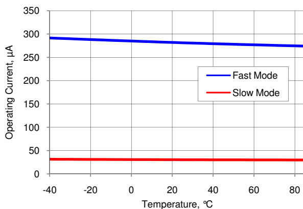
Figure 11-50. IDAC Operating Current vs Temperature, Range = 255 \mu A, Code = 0, Source Mode
