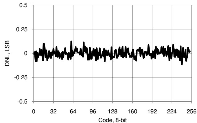
Figure 11-45. IDAC DNL vs Input Code, Range = 255 \mu A, Sink Mode
