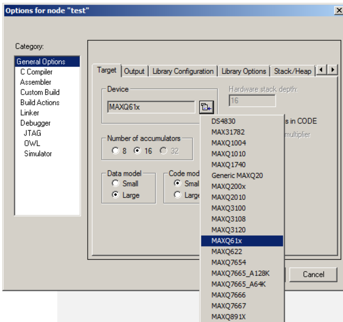
Figure 5. IAR Project Configuration
