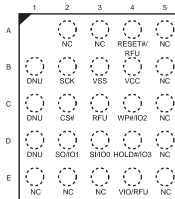
Figure 6.2 24-Ball BGA, 5 x 5 Ball Footprint (FAB024), Top View
