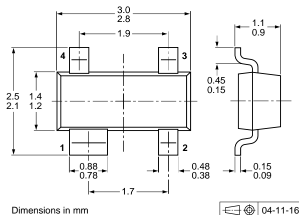
Fig 8. Package outline SOT143B
