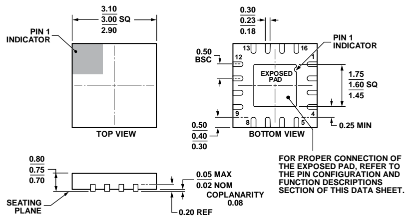
Figure 54. 16-Lead Lead Frame Chip Scale Package [LFCSP_WQ] 3 mm x 3 mm Body, Very Very Thin Quad (CP-16-22)
