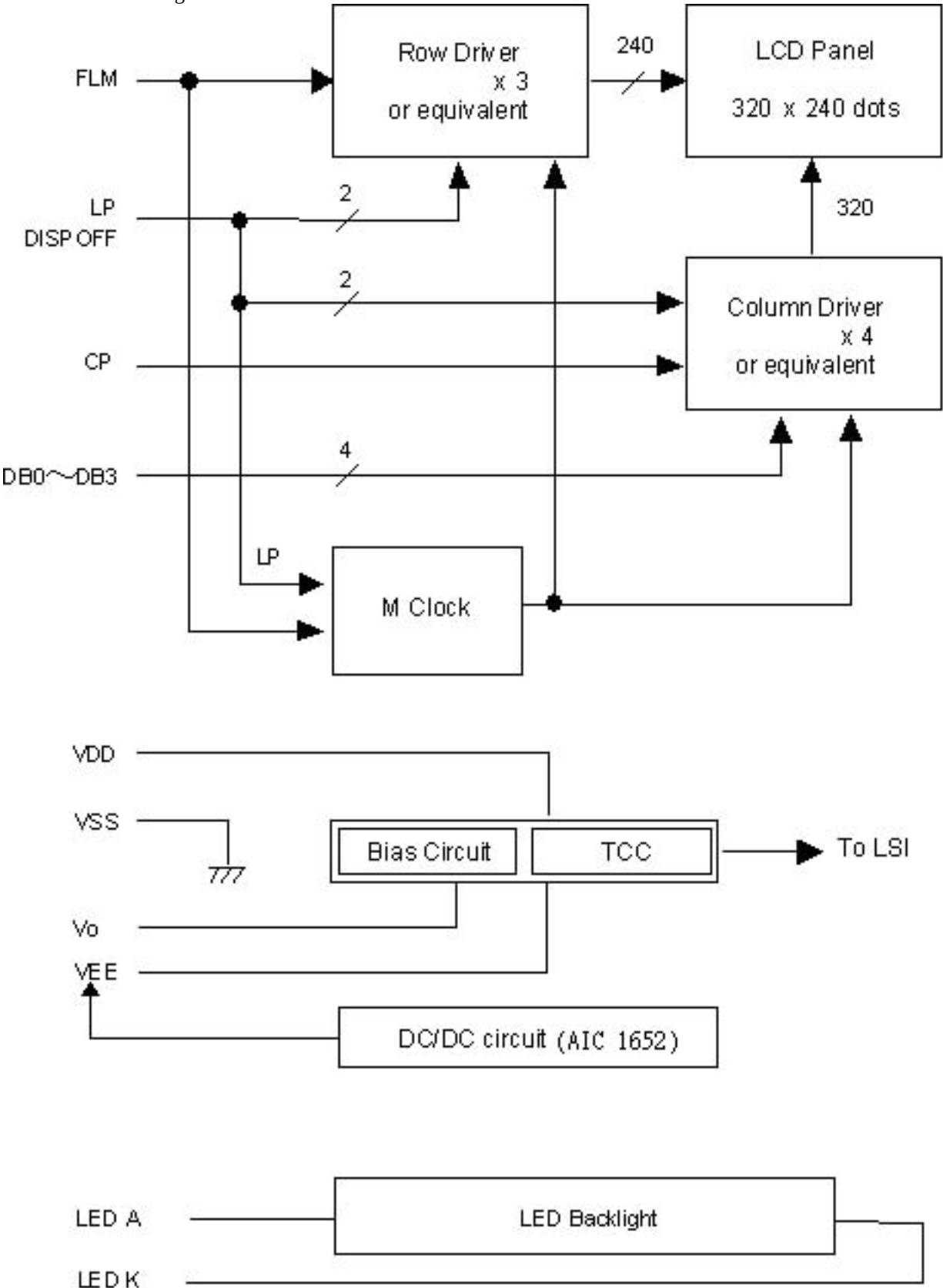
4.3 Block Diagram
