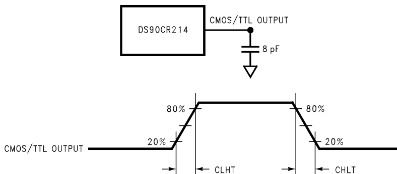
Figure 7. DS90CR214 (Receiver) CMOS/TTL Output Load and Transition Times
