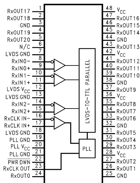
Figure 4. DS90CR214
