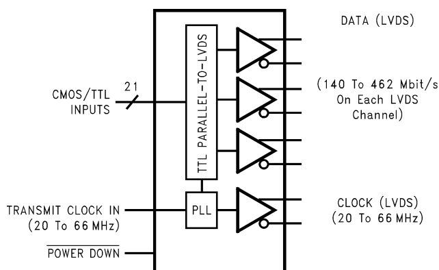
Figure 1. DS90CR213 See Package Number DGG0048A
