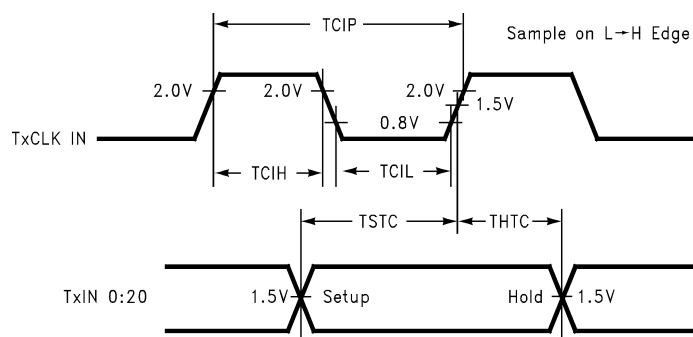
Figure 10. DS90CR213 (Transmitter) Setup/Hold and High/Low Times
