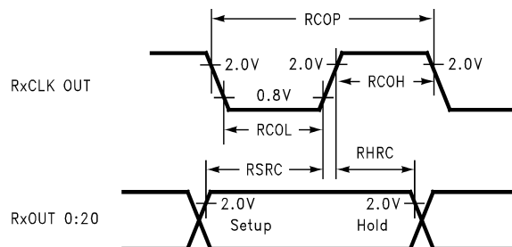
Figure 11. DS90CR214 (Receiver) Setup/Hold and High/Low Times
