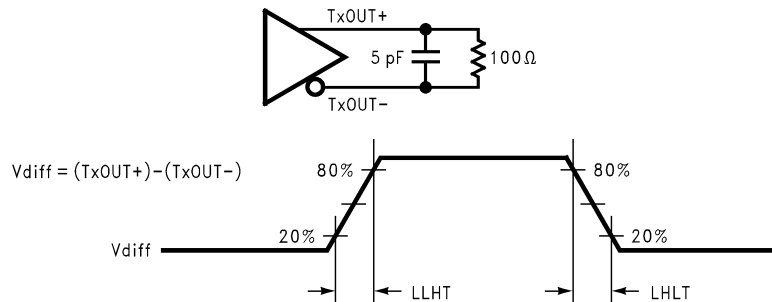
Figure 6. DS90CR213 (Transmitter) Input Clock Transition Time
