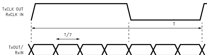
Figure 16. Seven Bits of LVDS in One Clock Cycle
