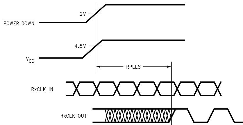
Figure 15. DS90CR214 (Receiver) Phase Lock Loop Set Time
