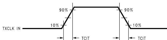
Figure 8. DS90CR213 (Transmitter) Input Clock Transition Time
