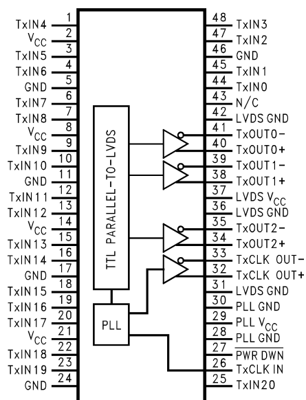
Figure 3. DS90CR213
