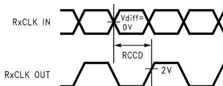
Figure 13. DS90CR214 (Receiver) Clock In to Clock Out Delay
