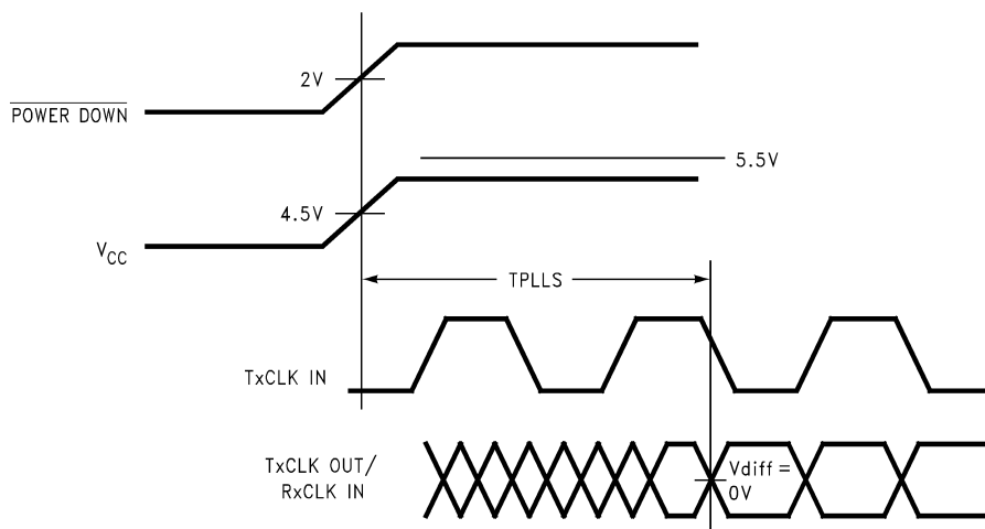
Figure 14. DS90CR213 (Transmitter) Phase Lock Loop Set Time
