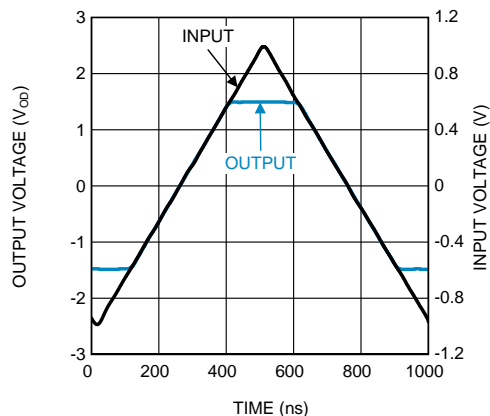
Figure 18. Overdrive Recovery
