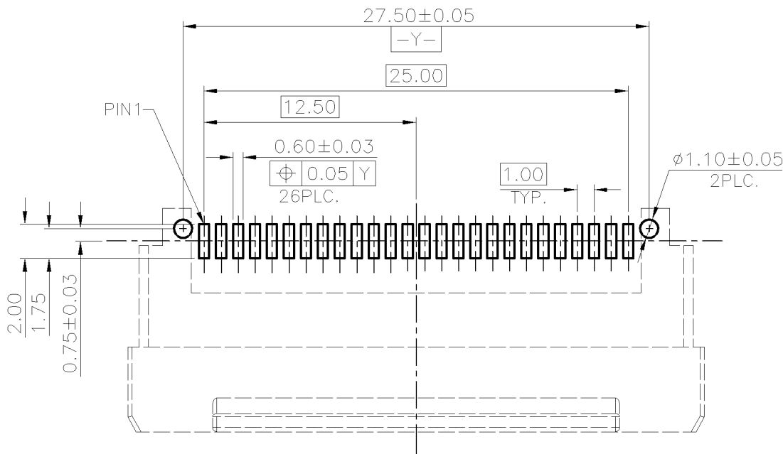
RECOMMENDED PCB LAYOUT CONNECTOR SIDE GENERAL TOLERANCE ±0.05
