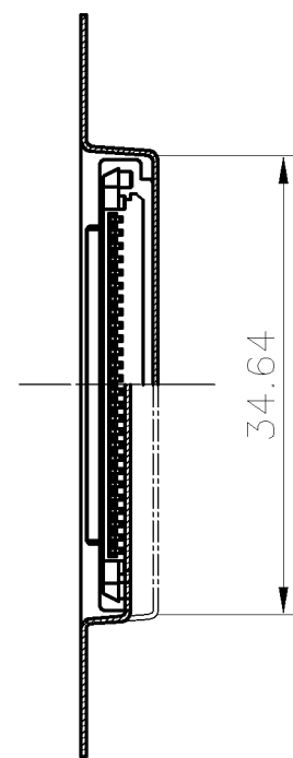
SECTION B-B
