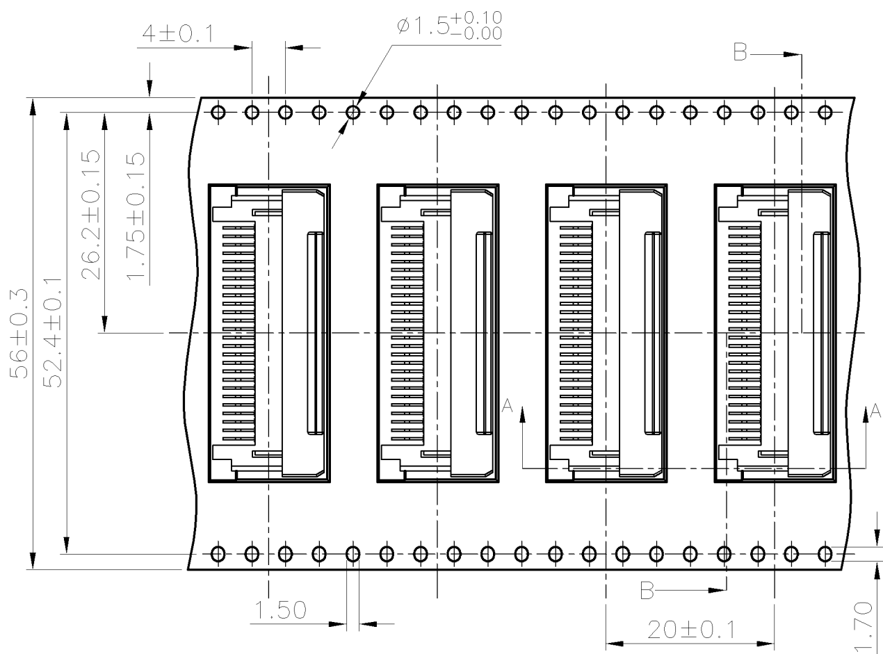
DETAIL X
