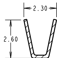
SECTION X-X
