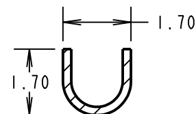
SECTION Y-Y
