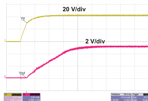
Figure 10. Top Converter Start-up relative to Vin, Vin=42V, Iout=1.5A
