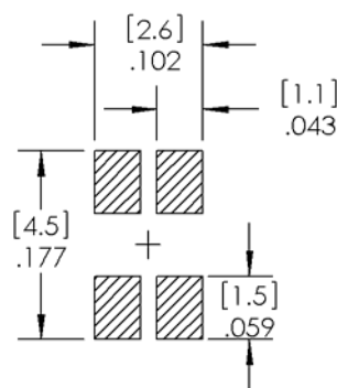
RECOMMENDED SOLDER PASTE PATTERN
