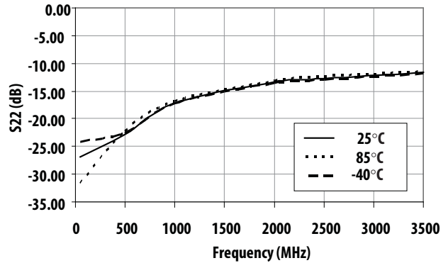
Figure 22. S22 (Return Loss) at Vctrl =5V vs Frequency vs Temperature
