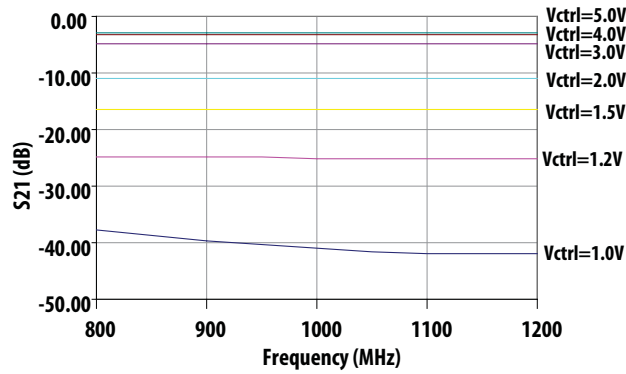
Figure 17. S21 Vs Frequency as function of Vctrl at Fc= 1GHz
