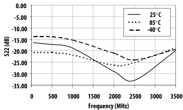
Figure 21. S22 (Return Loss) at Vctrl =1V vs Frequency vs Temperature
