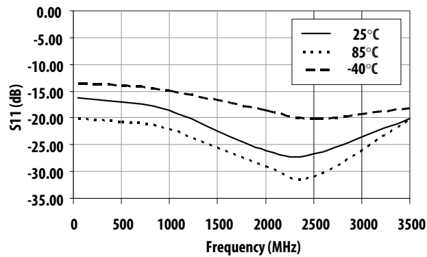
Figure 19. S11 (Return Loss) at Vctrl =1V vs Frequency vs Temperature
