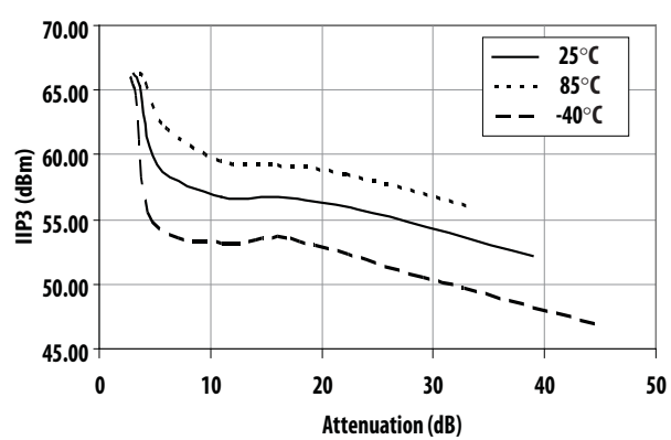
Figure 32. Input IP3 vs Attenuation vs Temperature at 1900MHZ
