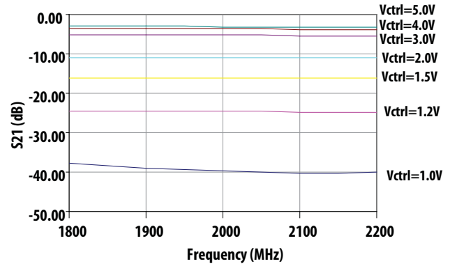
Figure 18. S21 Vs Frequency as function of Vctrl at Fc= 2GHz
