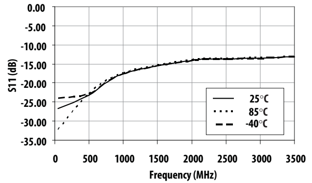
Figure 20. S11 (Return Loss) at Vctrl =5V vs Frequency vs Temperature
