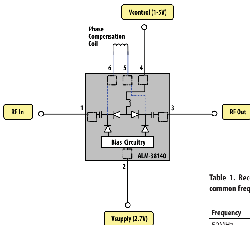
Figure 33. Simplified Schematic
