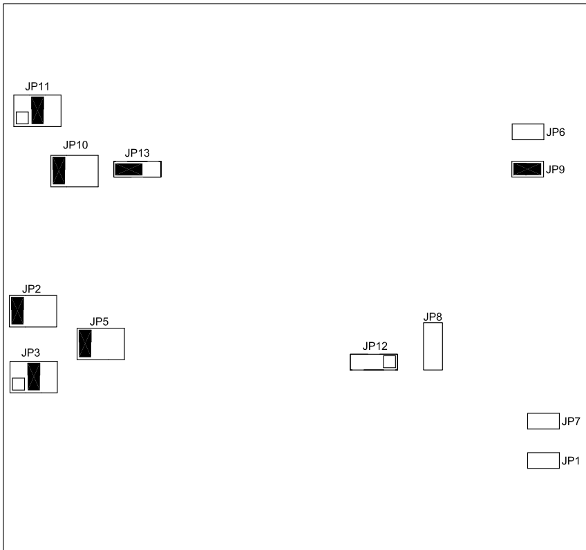
Figure 2-2. Jumper Locations
