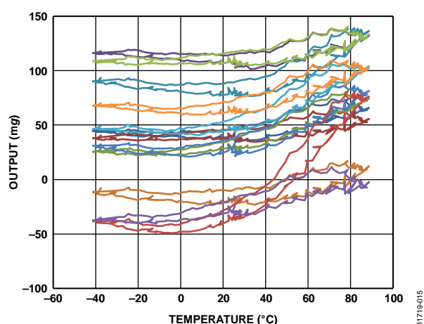
Figure 15. Accelerometer Z-Axis Zero g Offset vs. Temperature—16 Parts Soldered to PCB, ODR = 100 Hz, V_S = 2\text{ V}
