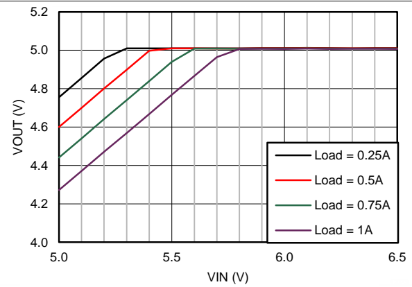
Figure 14. Drop-Out Curve
