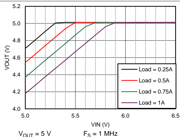
Figure 68. Drop-Out Curve
