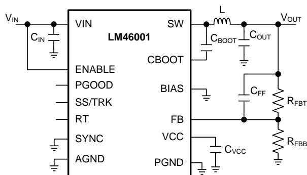
Figure 45. LM46001 Basic Schematic for V_{OUT} < 3.3\text{ V} , tie BIAS to Ground
