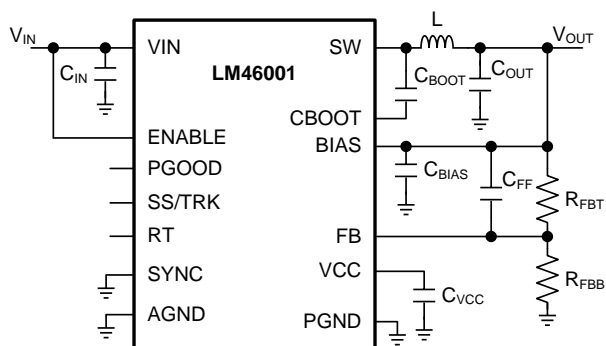
Figure 44. LM46001 Basic Schematic for V_{OUT} \geq 3.3\text{ V} , tie BIAS to V_{OUT}
