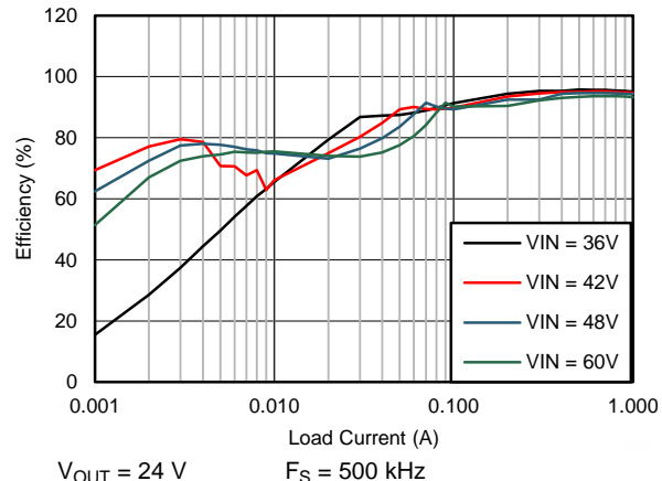
Figure 78. Efficiency
