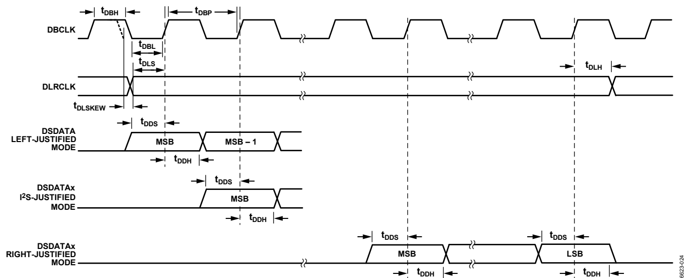
Figure 24. DAC Serial Timing
