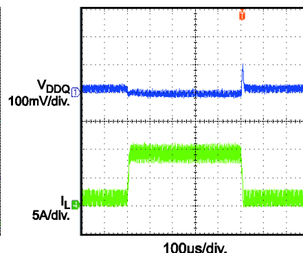
Transient I_O = 1 \sim 9A @ 1A/\mu s , F_{sw} = 500kHz C_O = 22\mu F \times 2 + 47\mu F
