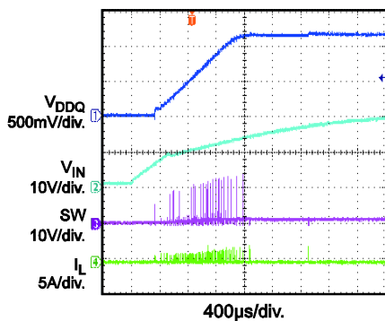
Start up through Vin I_O = 0A
