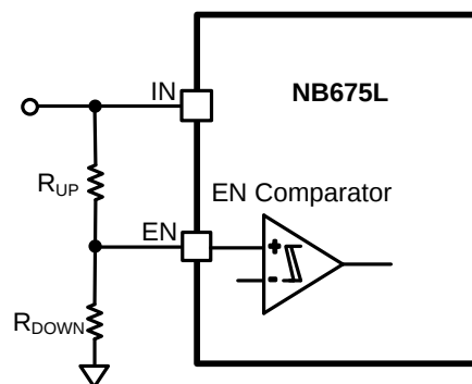
Figure 9—Adjustable UVLO
