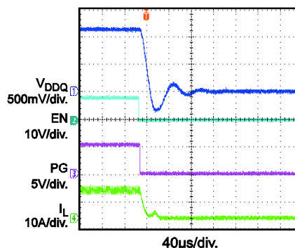
Power Good through EN Shutdown I_O = 10A
