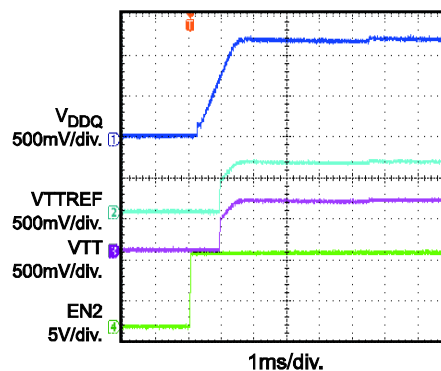
VTT&VTTREF Start-Up through EN2 I_O = 0A
