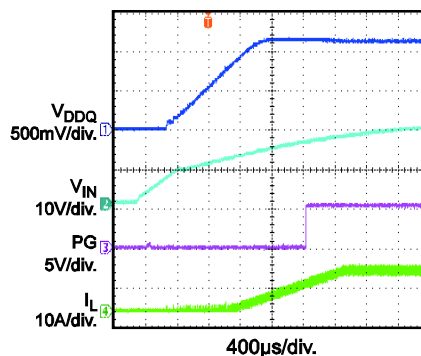
Power Good through Vin Start-up I_O = 10A
