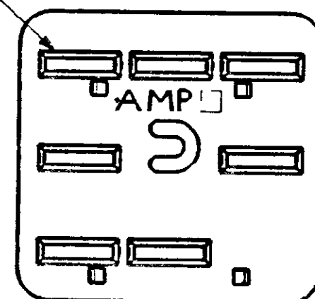
1-344085-9 (PINK) INHIB. VIEW
