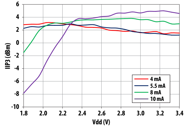
Figure 8. IIP3 vs. V_{dd}
