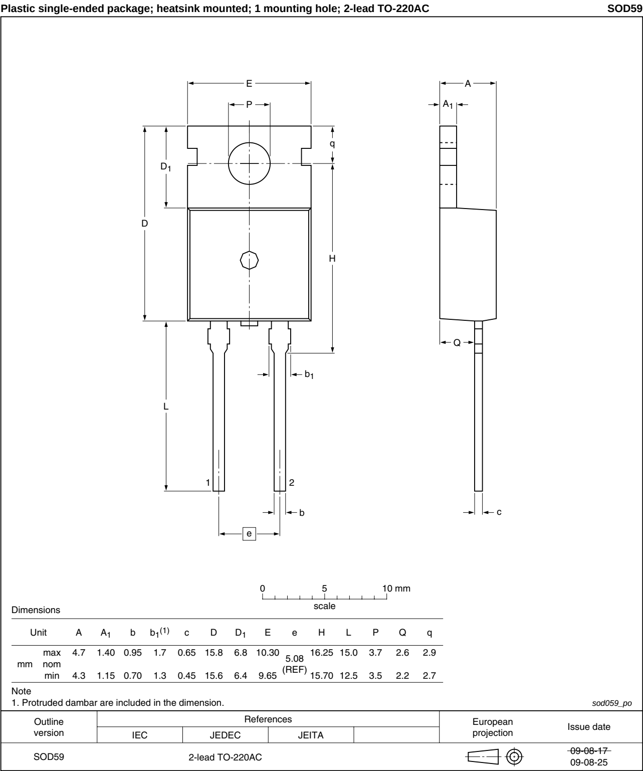
Fig 6. Package outline SOD59 (TO-220AC)
