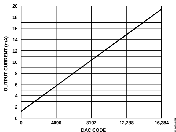
Figure 151. Gain Curve for FSC x[9:0] = 512 , DAC Offset = 1.228 mA
