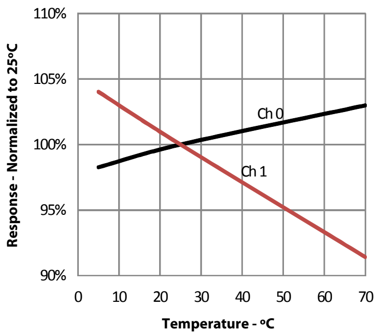
Figure TSL2591 – 15: Response to White LED vs. Temperature
