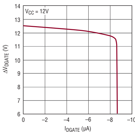
\Delta V_{\text{DGATE}} vs I_{\text{DGATE}}
