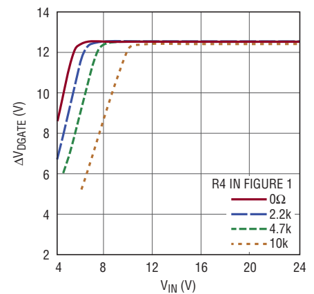
\Delta V_{\text{DGATE}} vs V_{IN} in Figure 1
