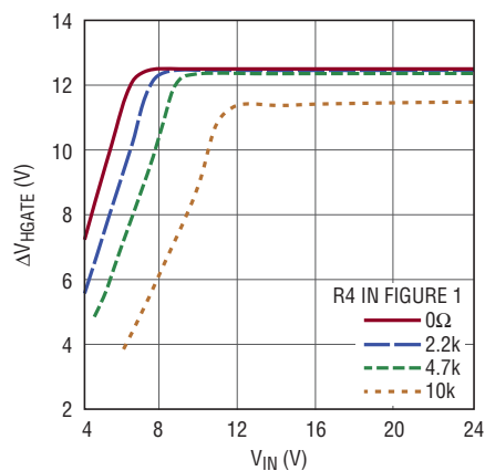
\Delta V_{\text{HGATE}} vs V_{IN} in Figure 1
