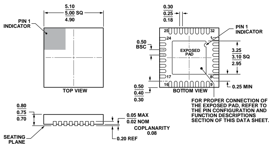
Figure 22. 32-Lead Frame Chip Scale Package [LFCSP_WQ] 5 mm × 5 mm Body, Very Very Thin Quad (CP-32-7)
