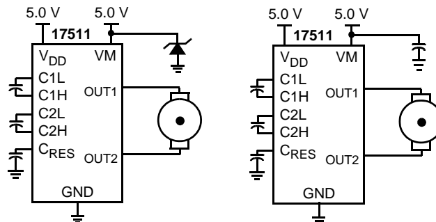
Figure 8. CEMF Snubbing Techniques
