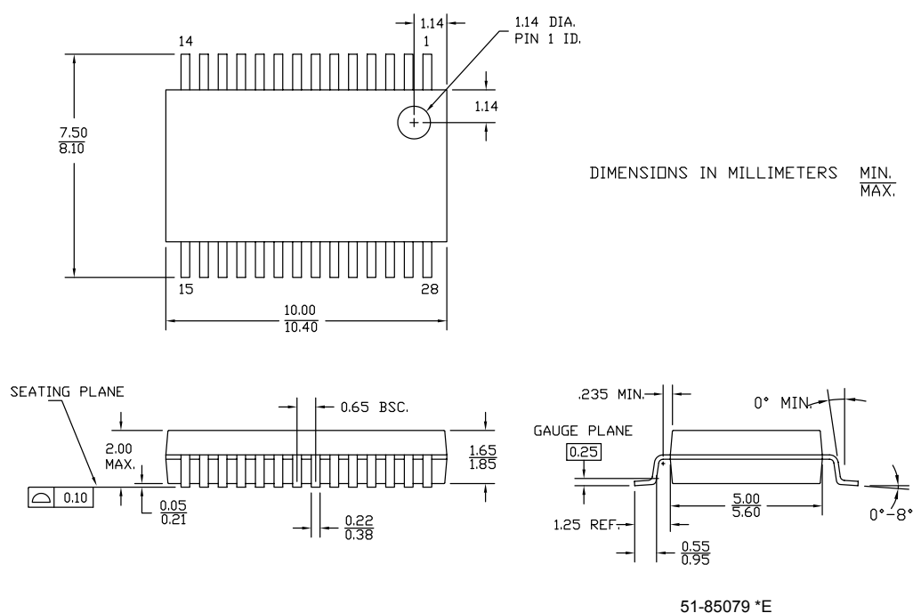
Figure 10. 28-pin SSOP (210 Mils) Package Outline, 51-85079
