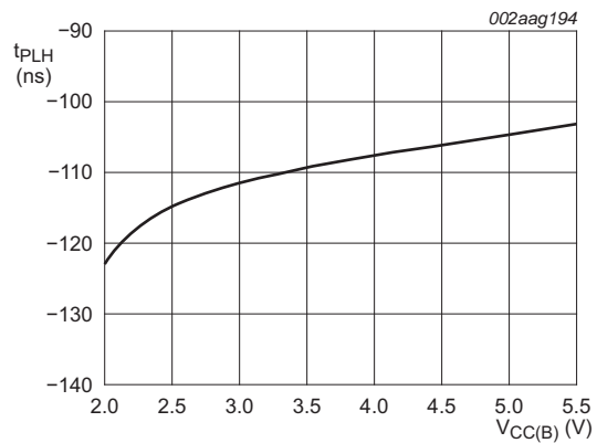
T_{amb} = 27\text{ }^{\circ}\text{C}; V_{CC(A)} = 1.1\text{ V}
