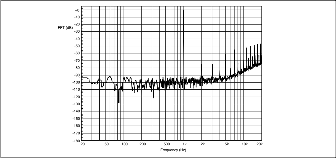
Figure 9. FFT performance (0 dBFS)
