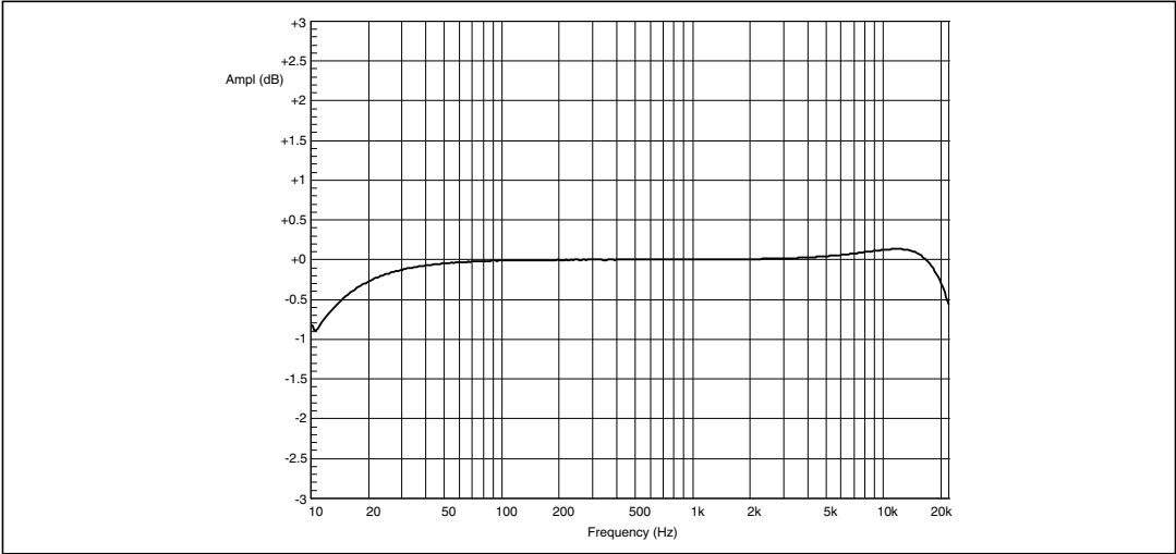
Figure 8. Frequency response
