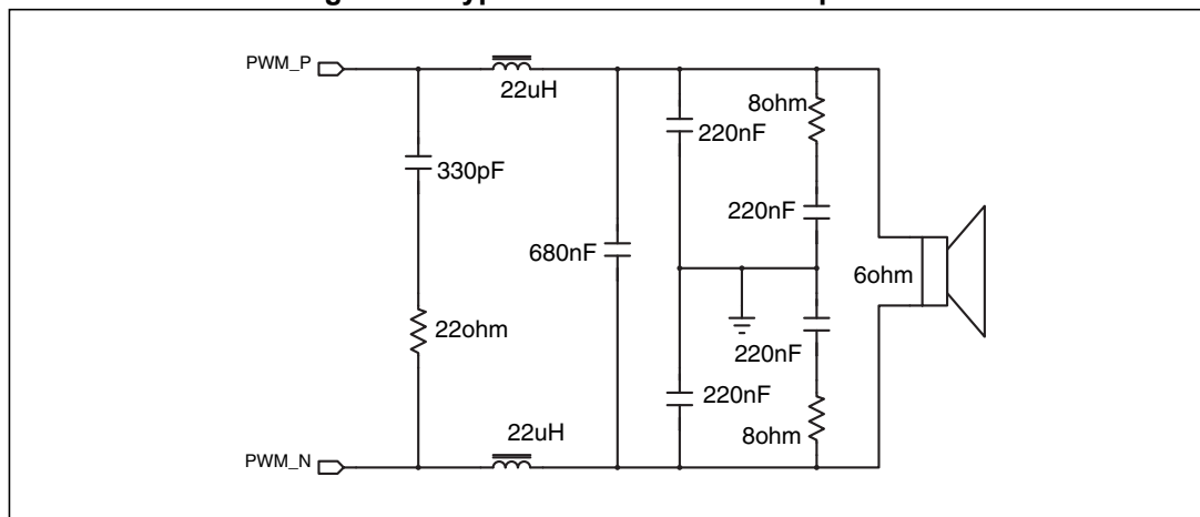
Figure 24. Typical LC filter for a 6 \Omega speaker
