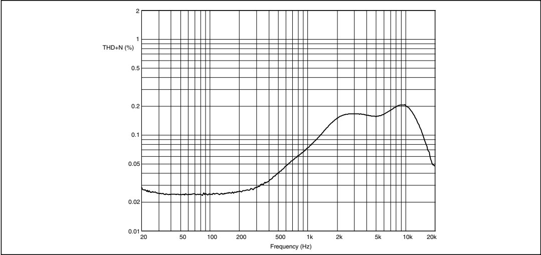
Figure 6. THD vs. frequency (1 W)
