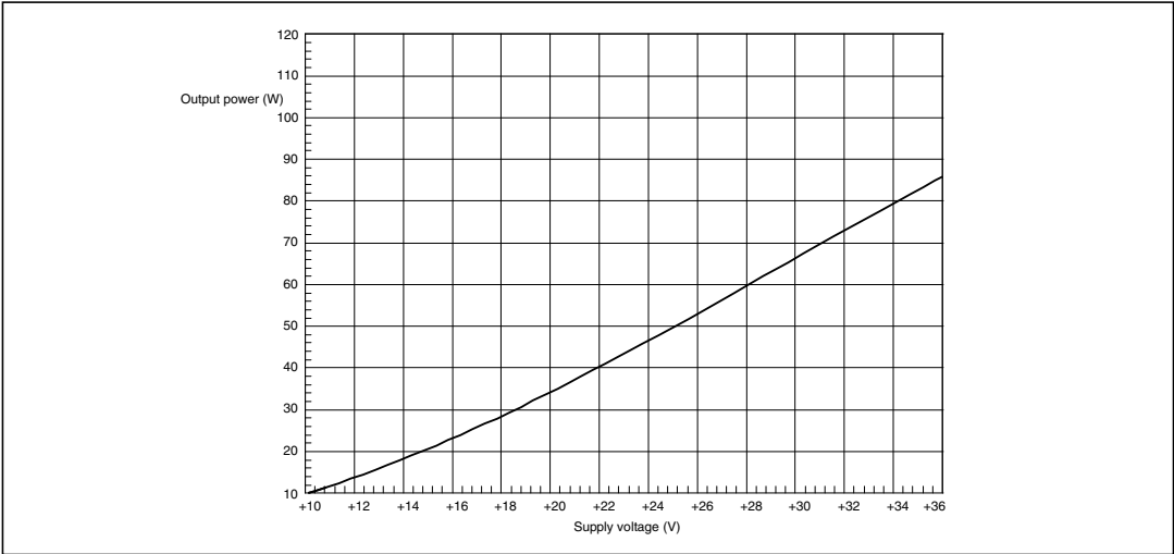
Figure 11. Output power (THD = 10%) vs. supply voltage
