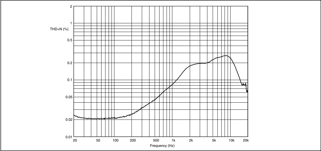
Figure 13. THD vs. frequency (1 W)
