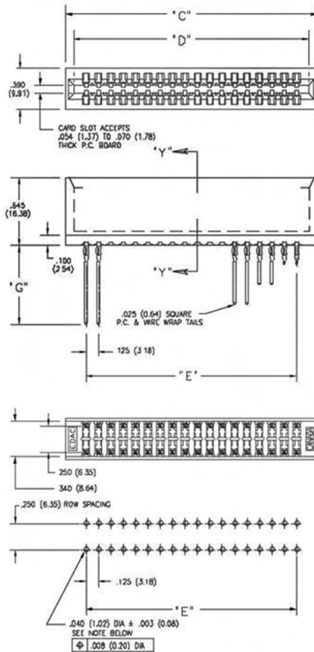
RECOMMENDED MOTHER BOARD HOLE PATTERN
